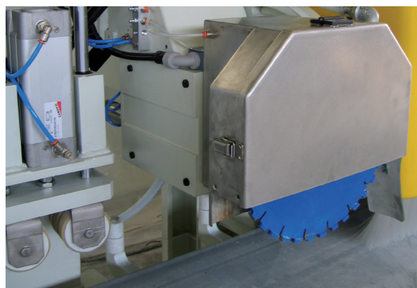
Drip cut unit Gocciolatoio
